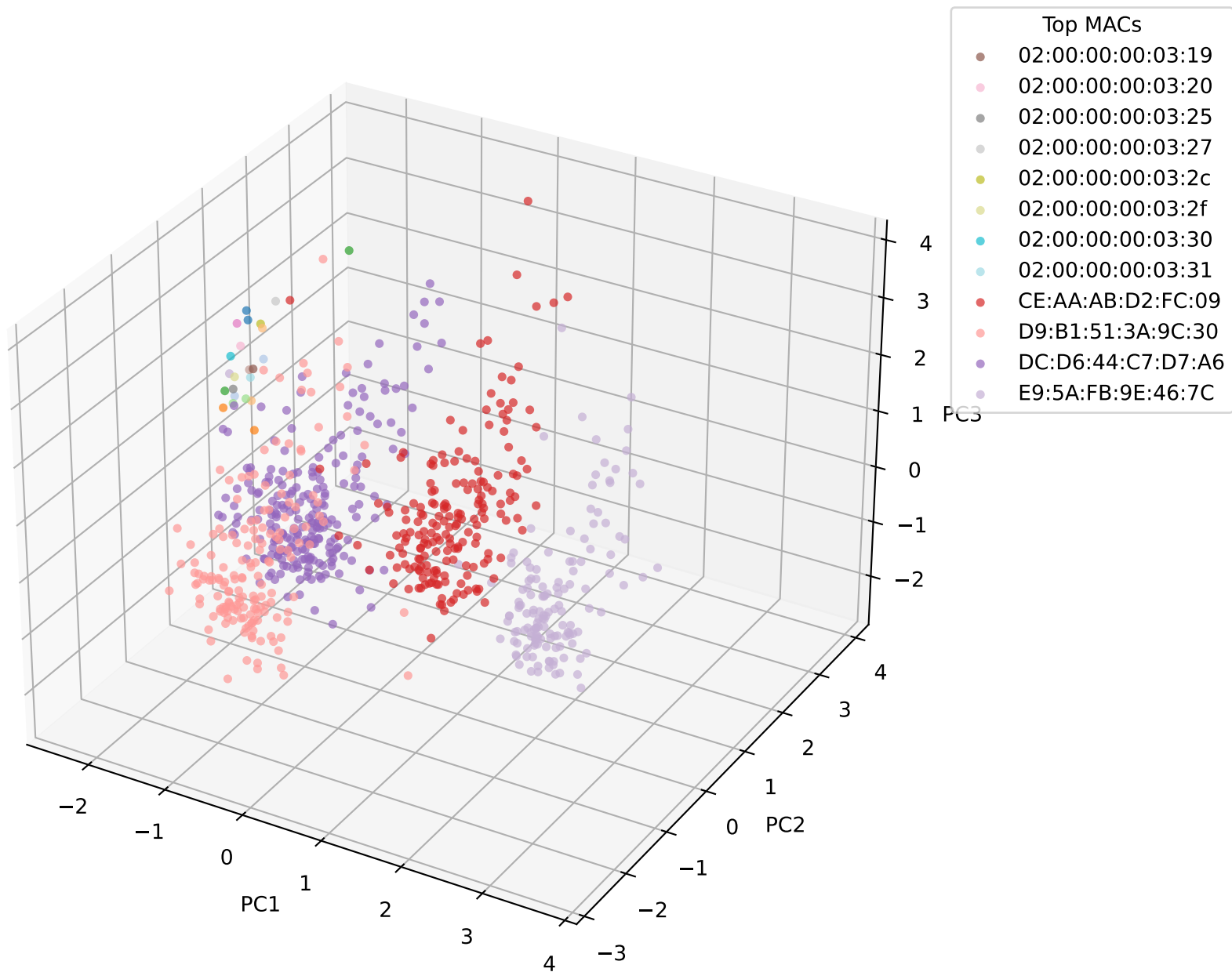
MAC-colored 3-D PCA of CFO (EVR: 0.38, 0.31, 0.23)
