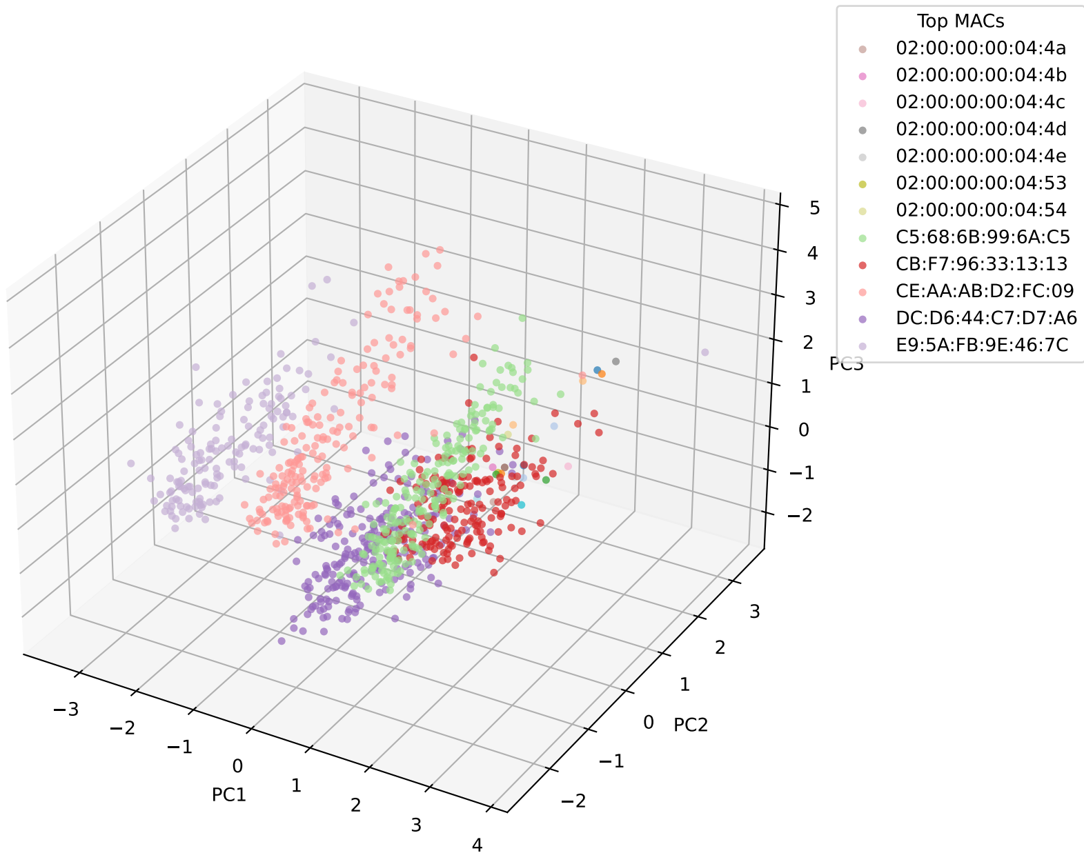
MAC-colored 3-D PCA of CFO (EVR: 0.36, 0.31, 0.23)
