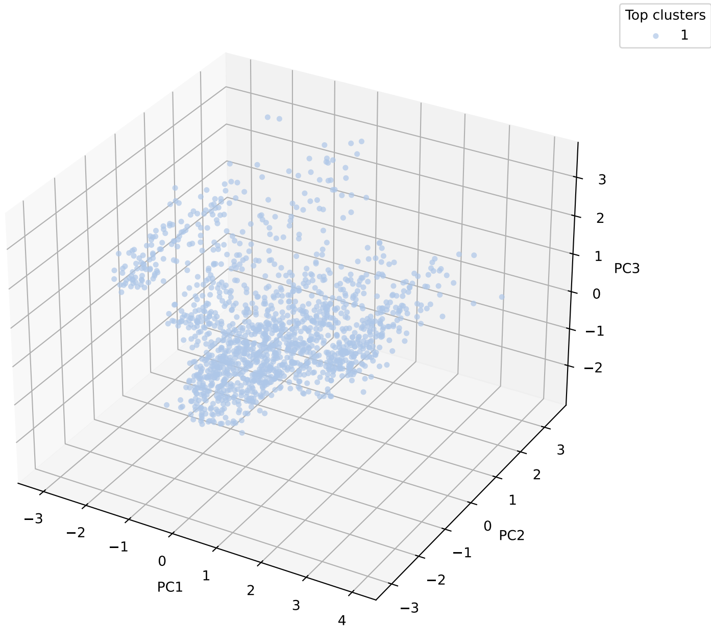
Clusters in 3-D PCA space (EVR: 0.35, 0.32, 0.24)
