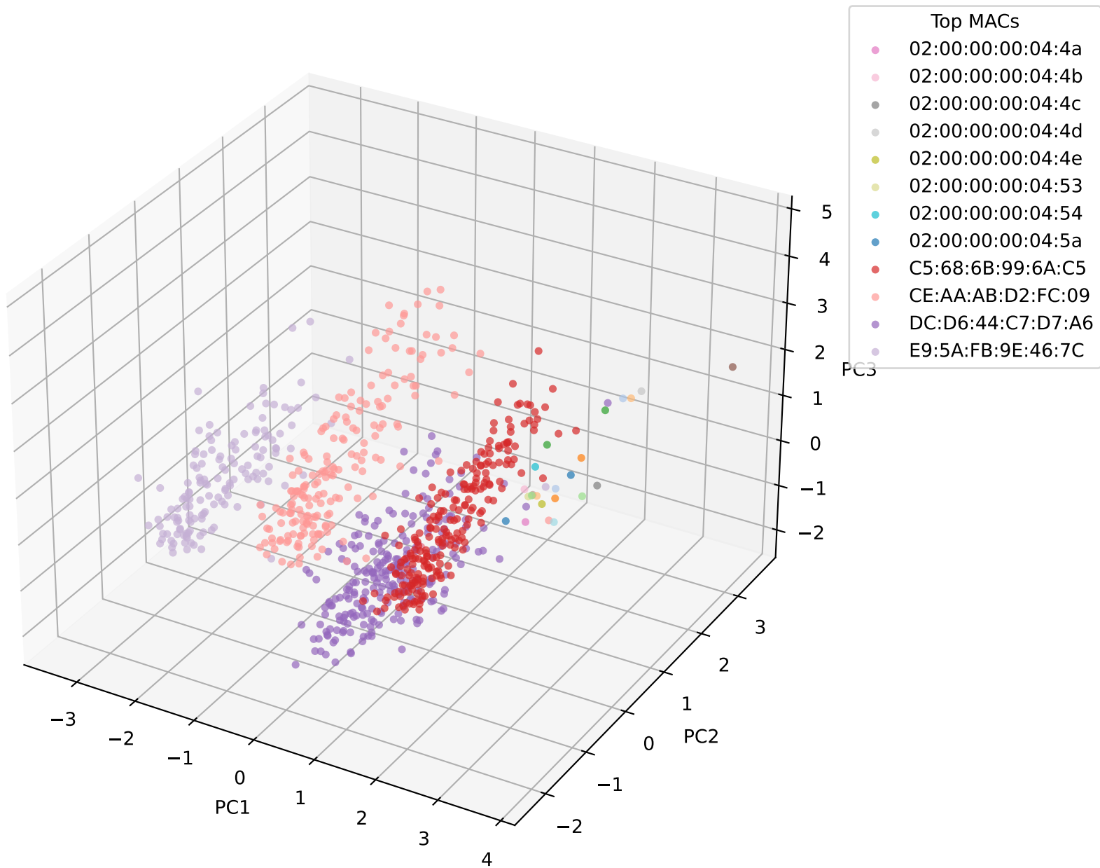
MAC-colored 3-D PCA of CFO (EVR: 0.37, 0.31, 0.22)
