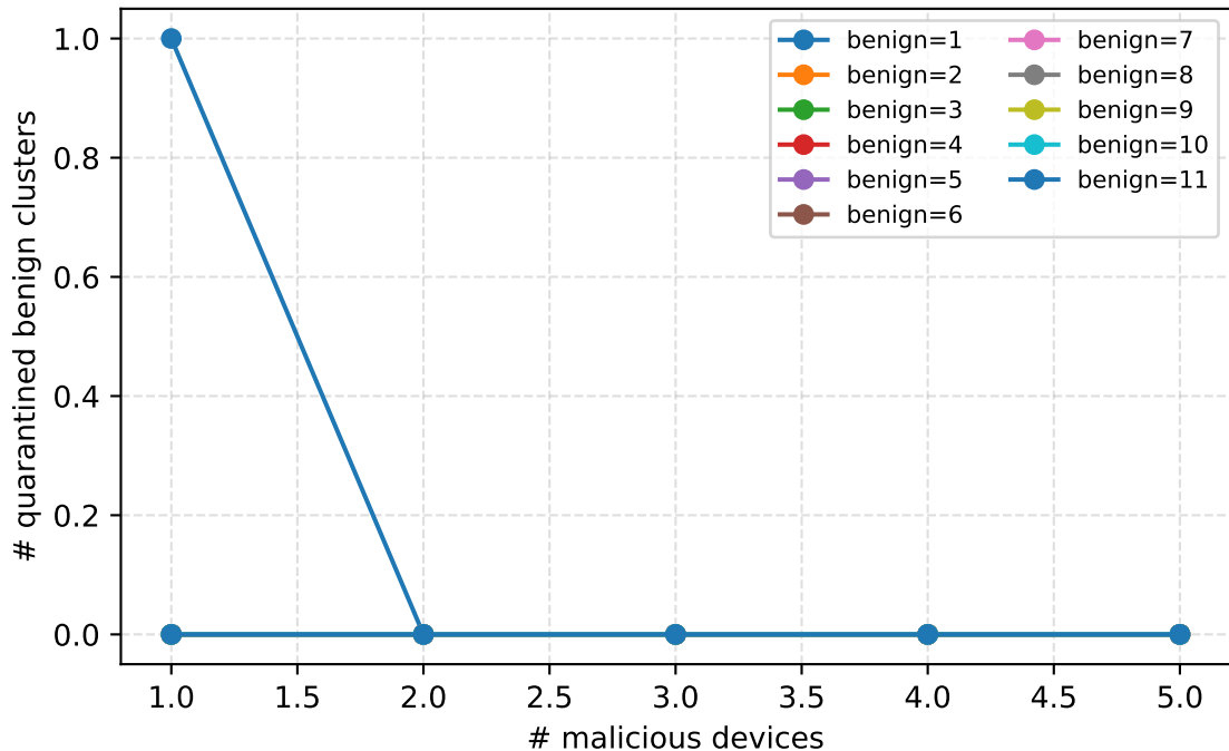
Benign quarantine effectiveness vs attackers
