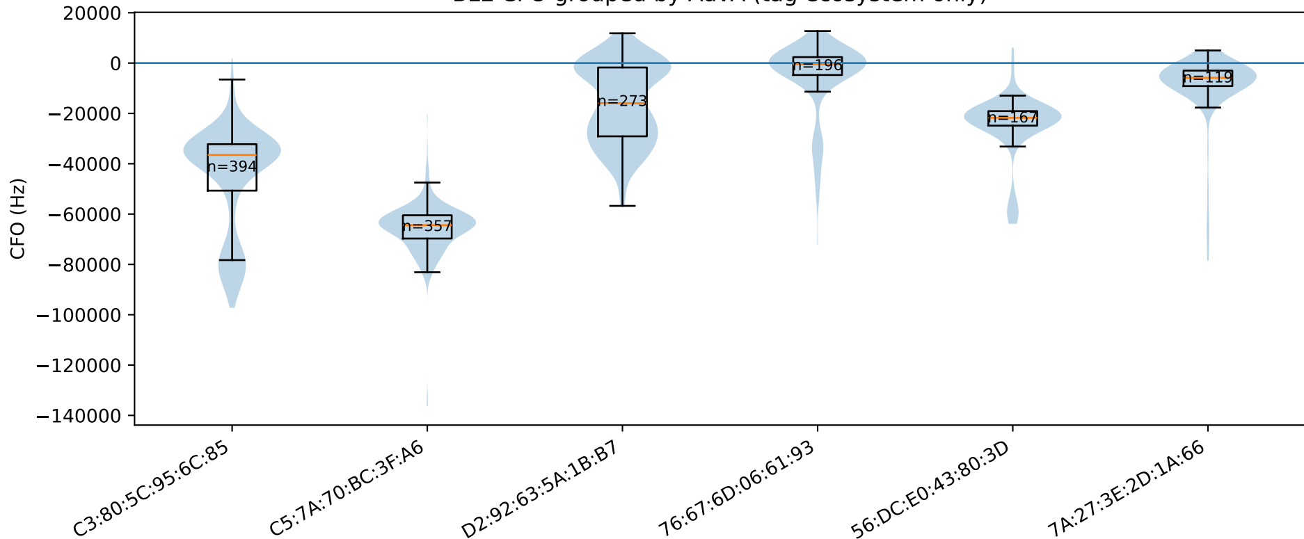
BLE CFO grouped by AdvA (tag ecosystem only)
