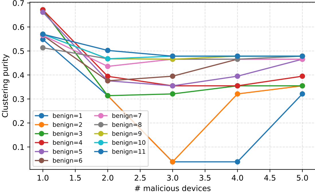
AirCatch clustering accuracy vs attackers
