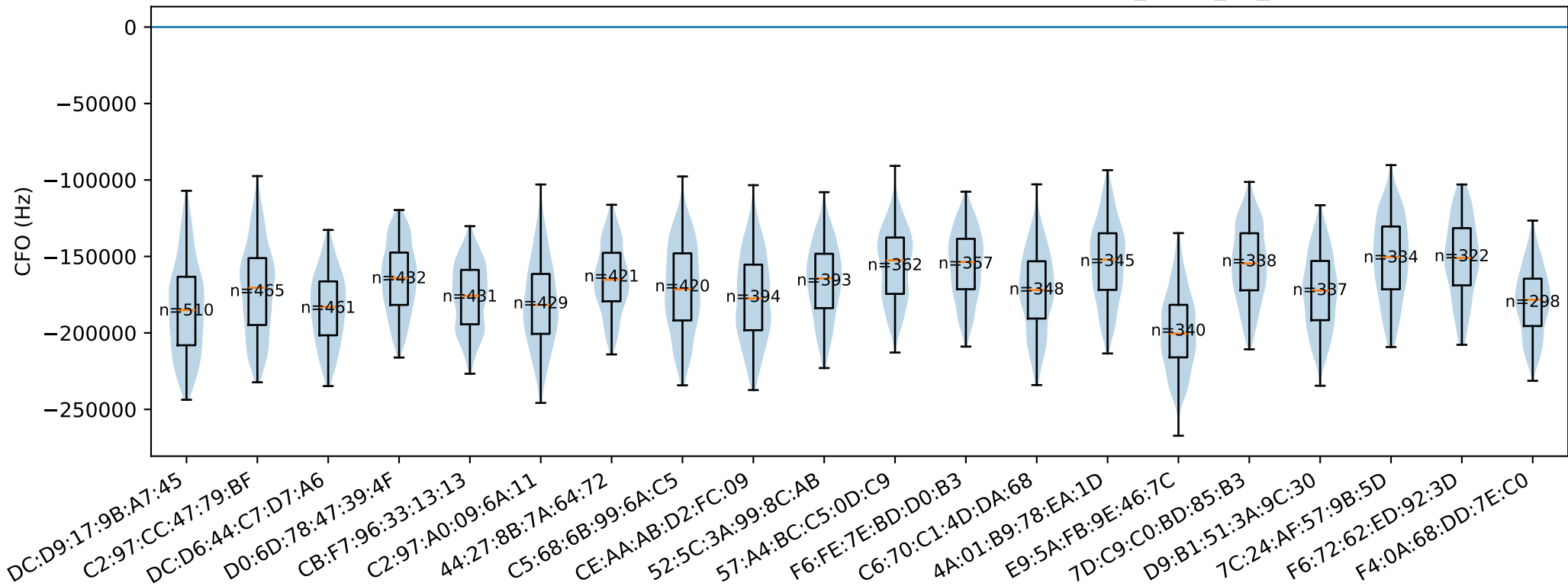
Transition CFO grouped by AdvA (tag ecosystem only): cfo_equal_11_hz
