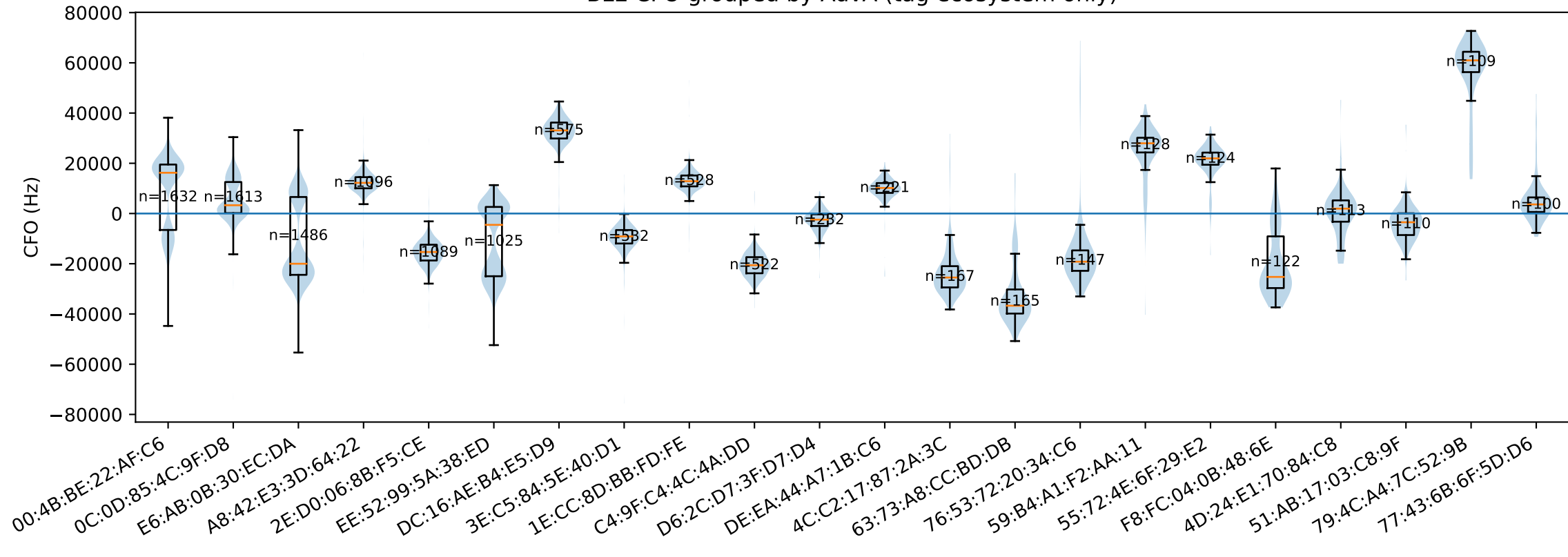
BLE CFO grouped by AdvA (tag ecosystem only)
