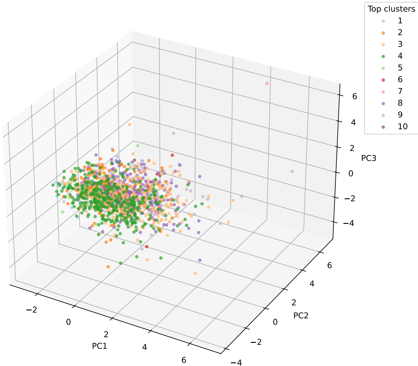
Clusters in 3-D PCA space (EVR: 0.40, 0.27, 0.14)
