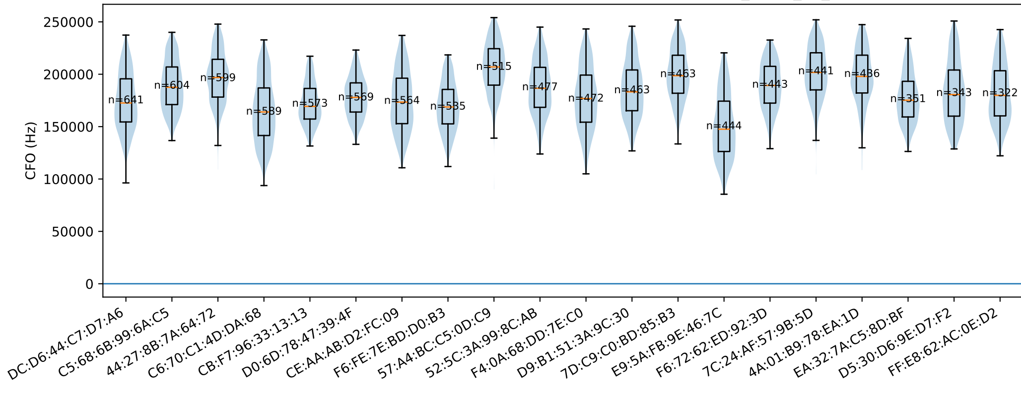
Transition CFO grouped by AdvA (tag ecosystem only): cfo_equal_00_hz
