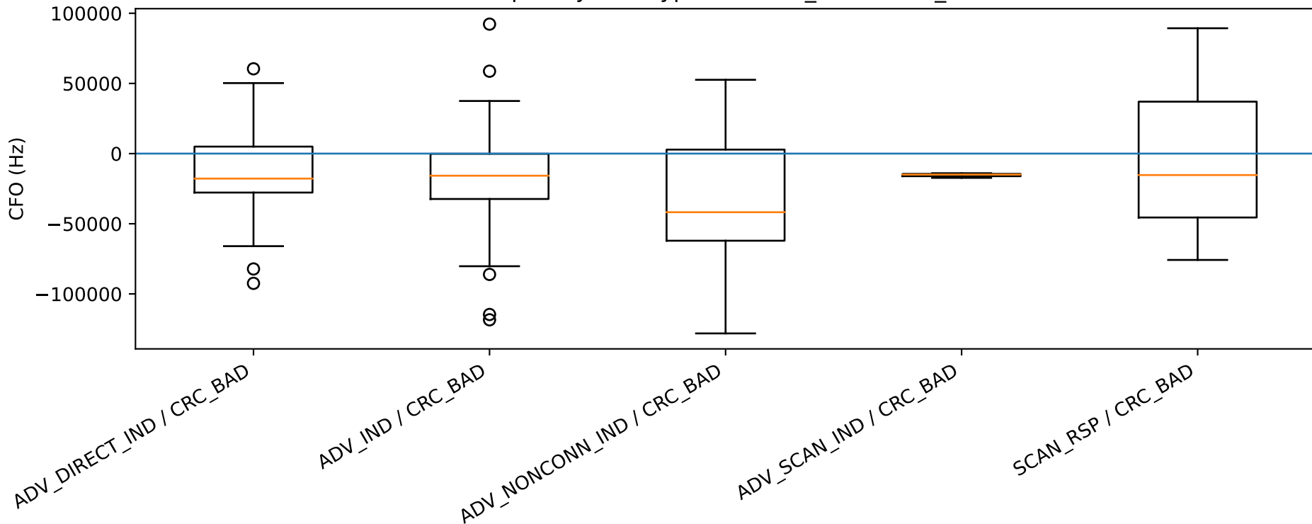
BLE CFO per decoded candidate (preamble→AA→header+payload, CRC excluded) Grouped by PDU type and CRC_OK vs CRC_BAD
