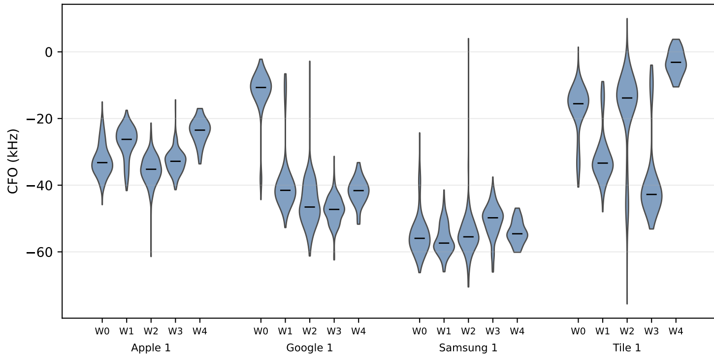
CFO drift as per-window distributions (15-min windows)
