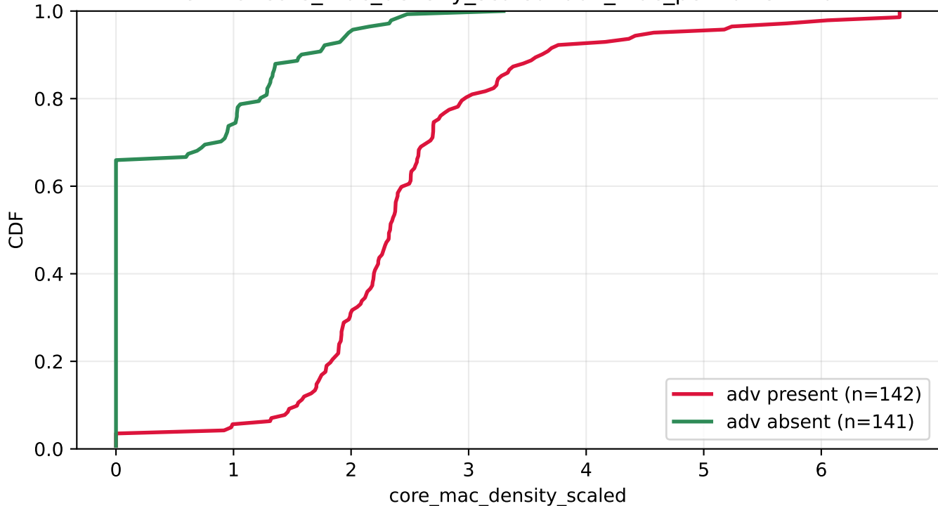
CDF of core_mac_density_scaled: adv_mac_pct>0 vs ==0
