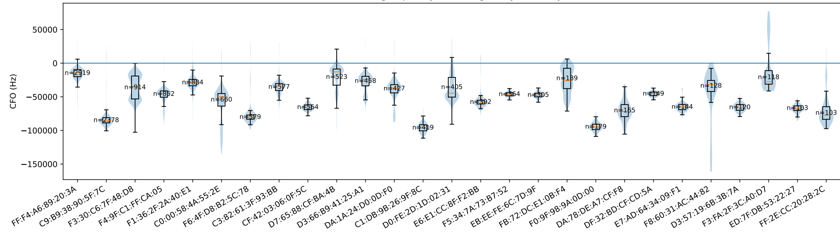
BLE CFO grouped by AdvA (tag ecosystem only)
