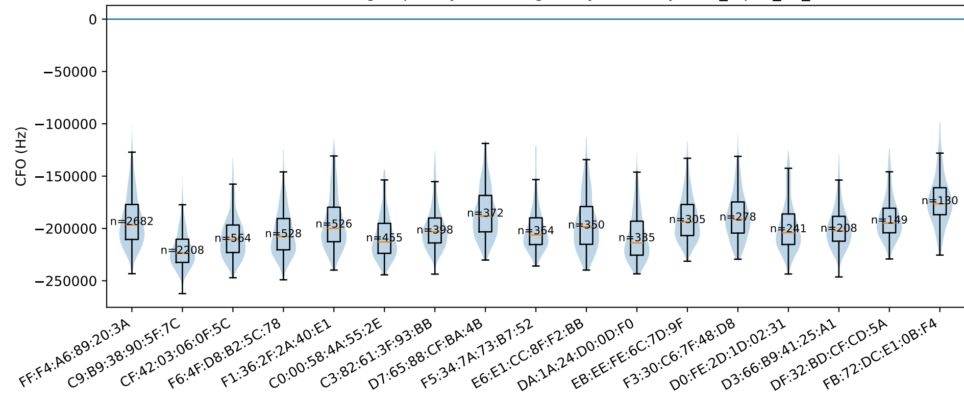
Transition CFO grouped by AdvA (tag ecosystem only): cfo_equal_11_hz
