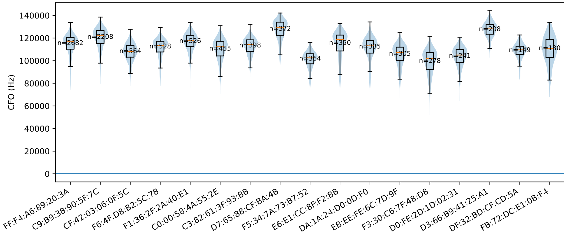
Transition CFO grouped by AdvA (tag ecosystem only): cfo_jump_10_hz
