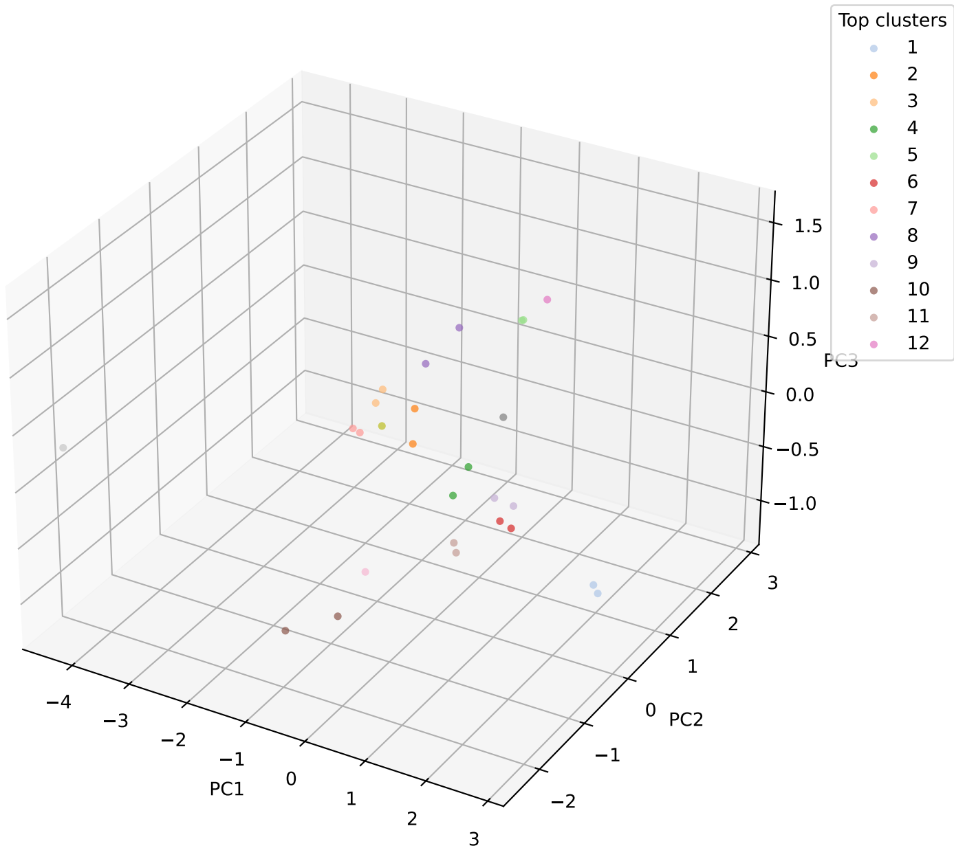
Clusters in 3-D PCA space (EVR: 0.46, 0.33, 0.09)
