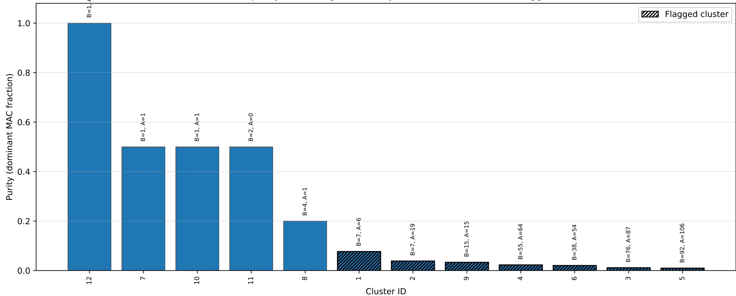
Cluster purity with benign/adversary MAC counts (hatched = flagged)
