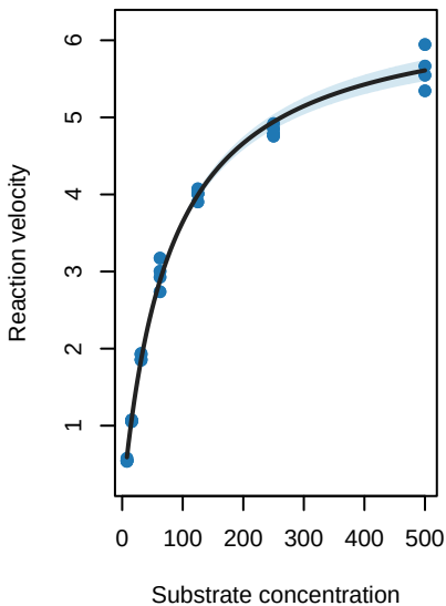
enzyme=1111 Var = gamma S 0.85
