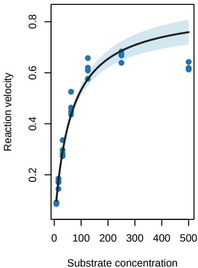
enzyme=4444 Var = gamma S 1
