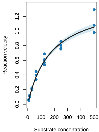
enzyme=2222 Var = gamma S 1
