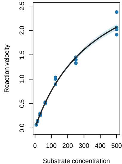
enzyme=3333 Var = gamma S 1
