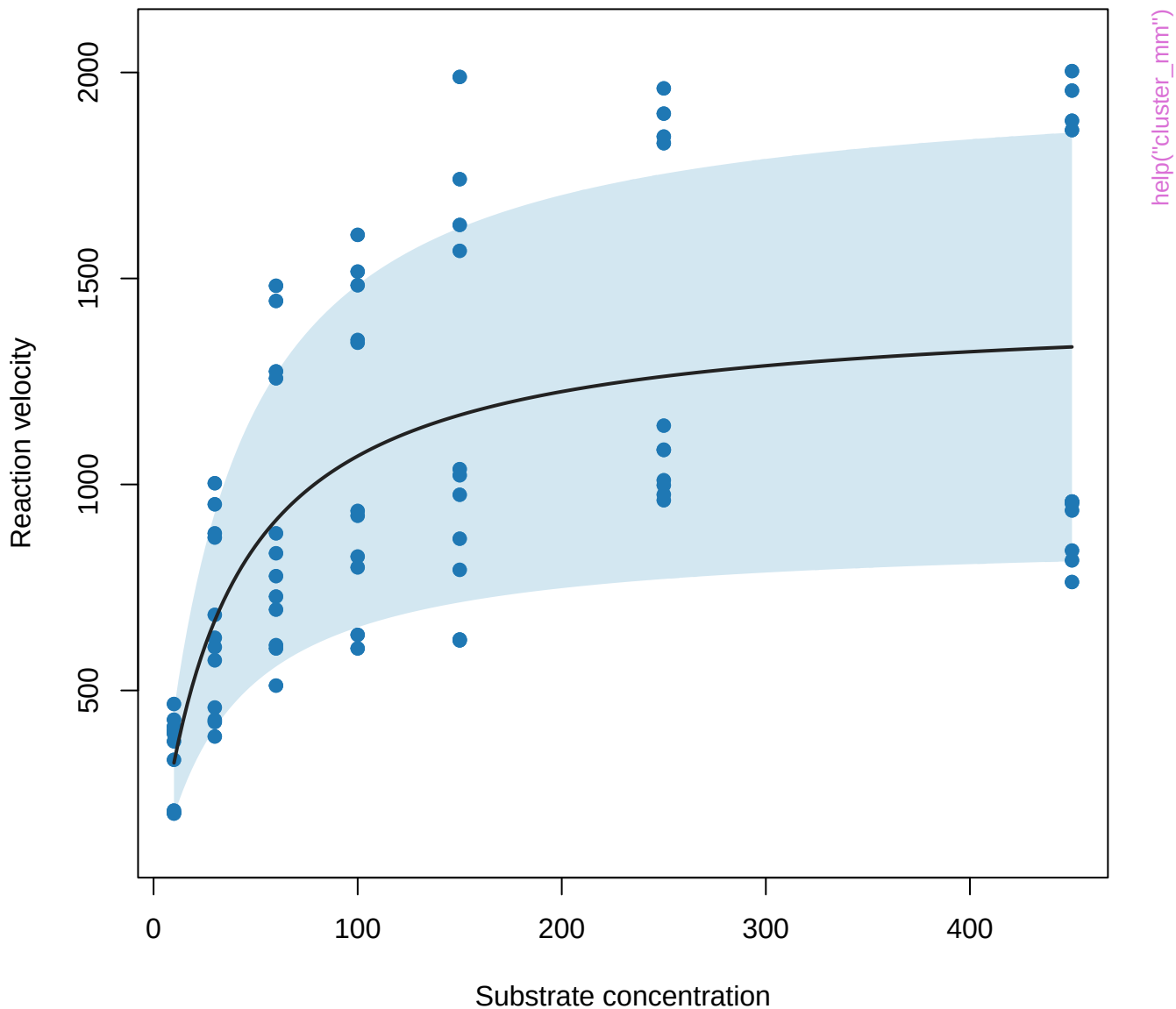
Clustered fit: \text{Var} = \gamma S^{(1/2)}
