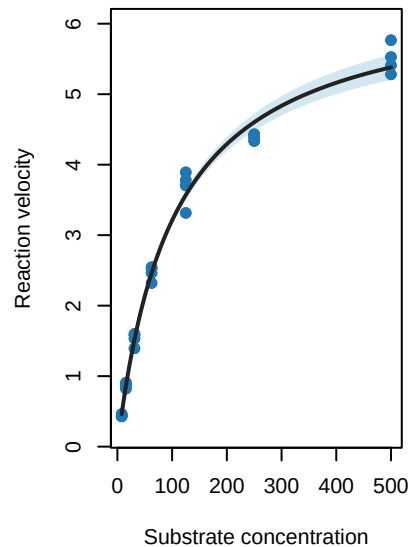
enzyme=6666 Var = gamma S 1
