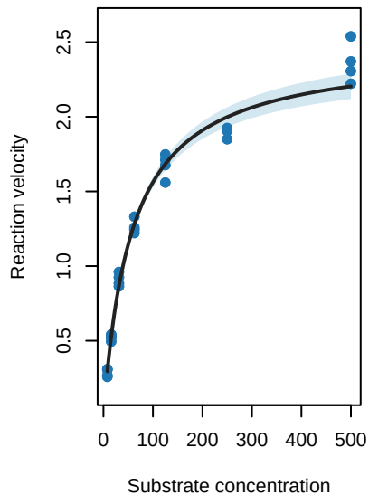
enzyme=5555 Var = gamma S 1
