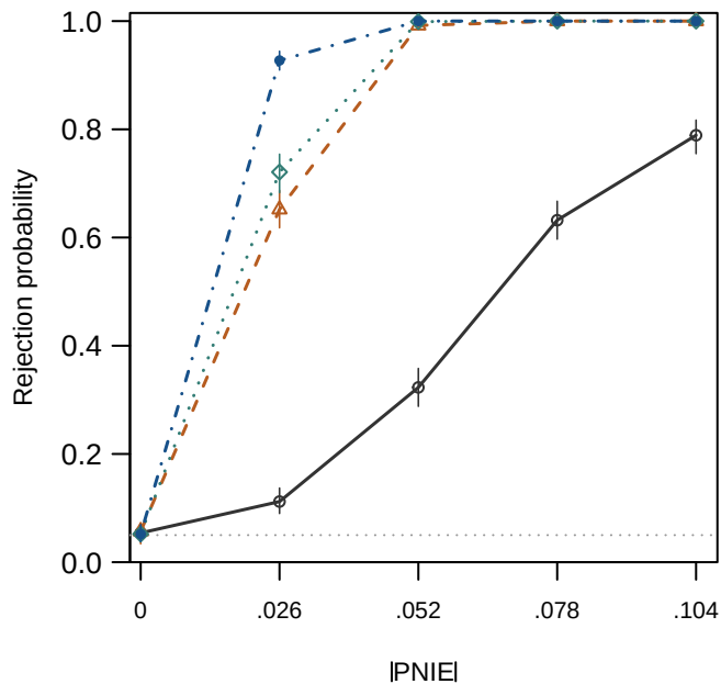
(b) Null-calibrated cutoff
