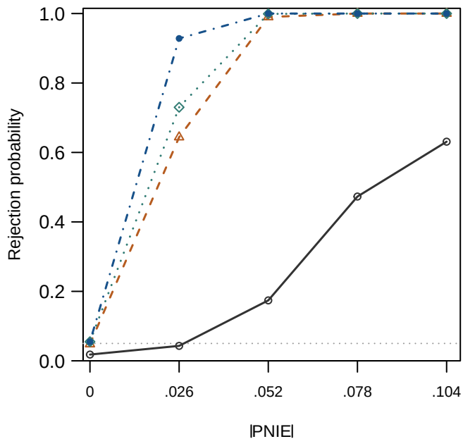
(a) Nominal cutoff
