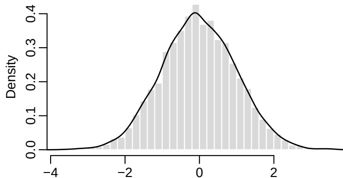
Gaussian
