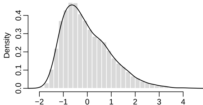
Skew-normal
