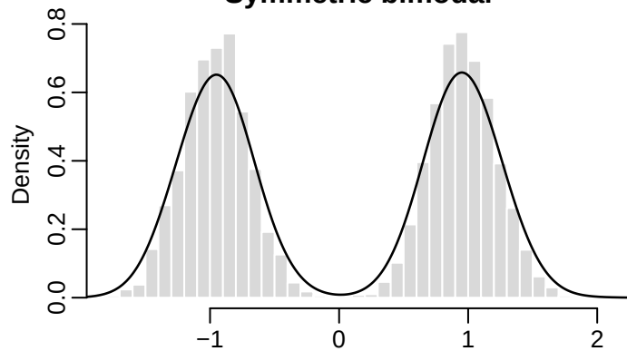
Symmetric bimodal
