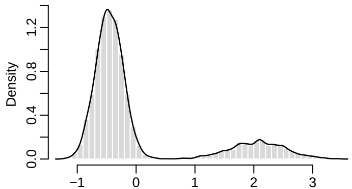
Asymmetric mixture
