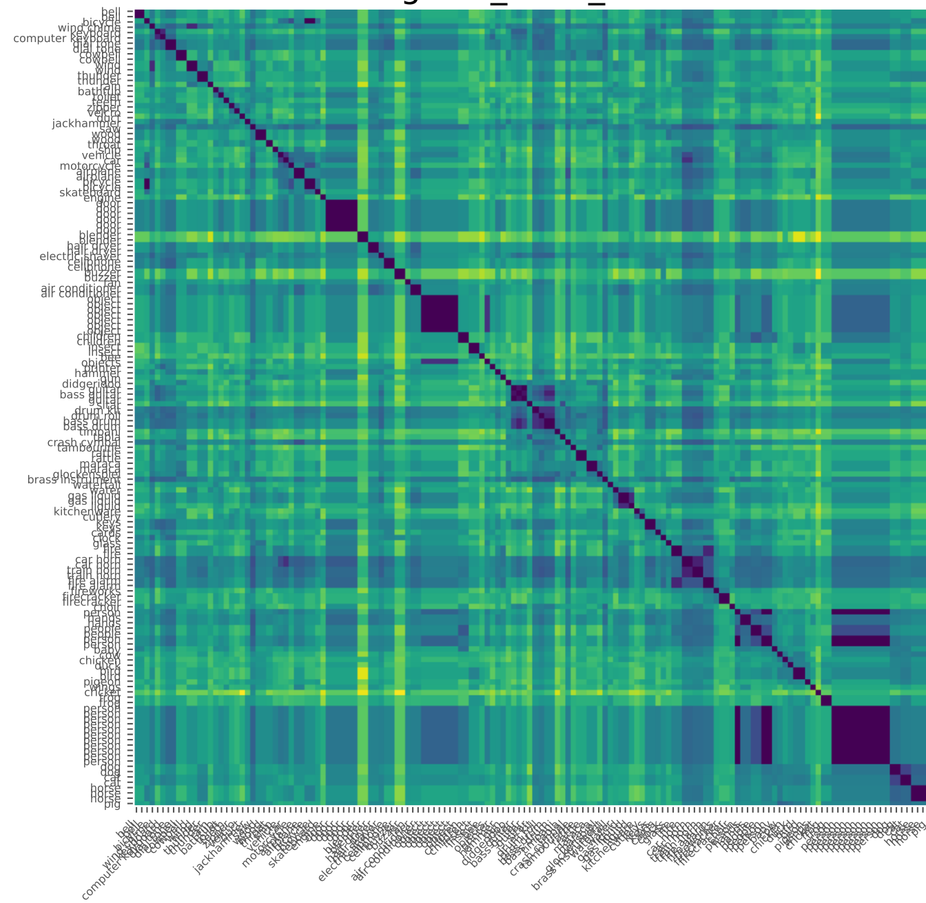
glove_what_euc
