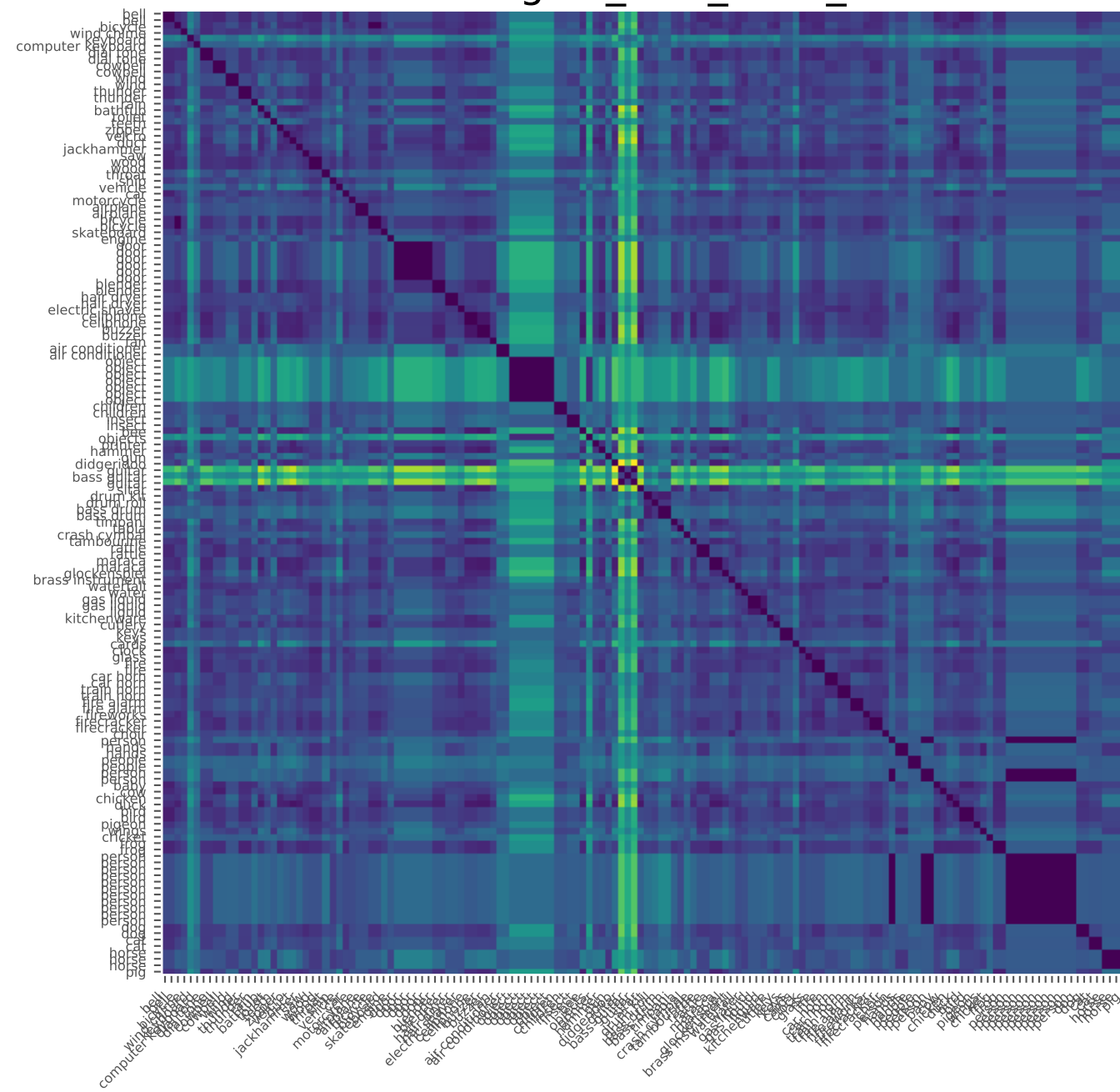
multilingual_bert_what_euc
