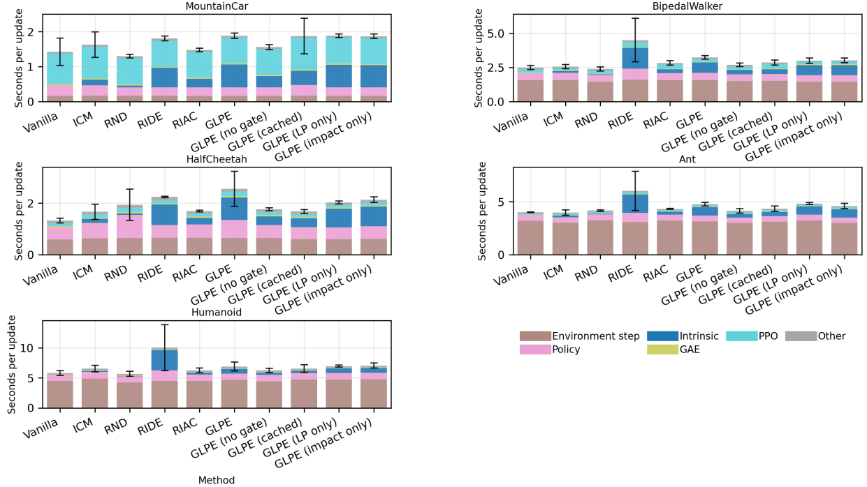
Figure 5.7: Runtime breakdown per PPO update. Each stack reports component-wise median time from the final quarter of training updates, averaged across runs. Black error bars show 95% confidence intervals for total update time across runs.
