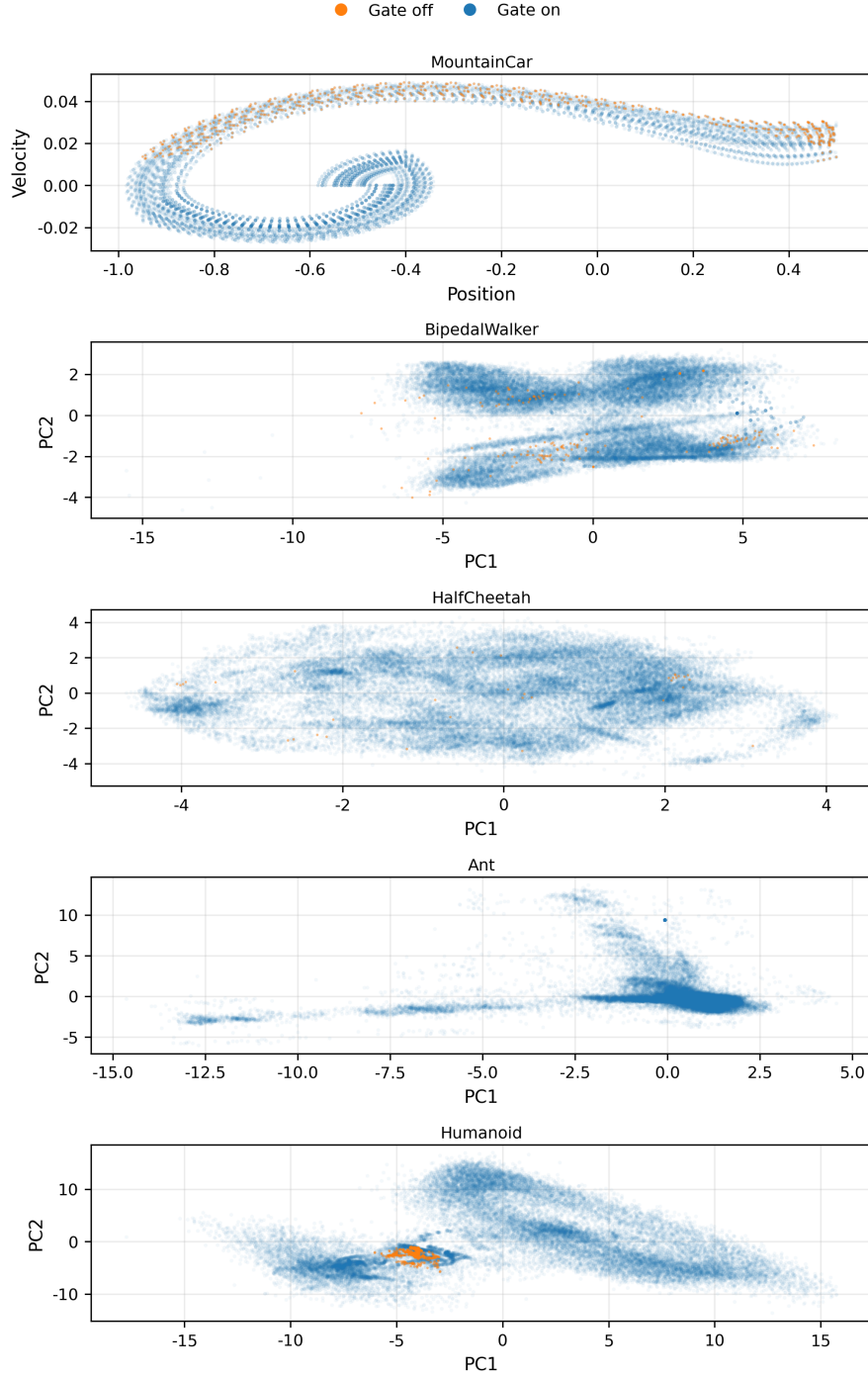
Figure 6: State-space view of GLPE’s gating decisions. Points are states visited in trajectories from the final checkpoint (subsamped); for MOUNTAINCAR-V0 we plot raw position and velocity, and for the remaining environments we project z-scored observations onto the first two principal components. Blue points indicate timesteps where the intrinsic term is active (gate on), while orange points indicate where the gate disables intrinsic shaping (gate off). Across tasks, gate-off points occupy a small and typically localized subset of the visited distribution, indicating that gating suppresses intrinsic shaping only in narrow regions rather than globally.
