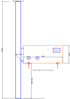
DUO (2) x 500 mm (base plate)
