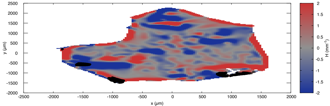
Face 5 (550_1_1) --- Mean Curvature H with Detected Anomalies
