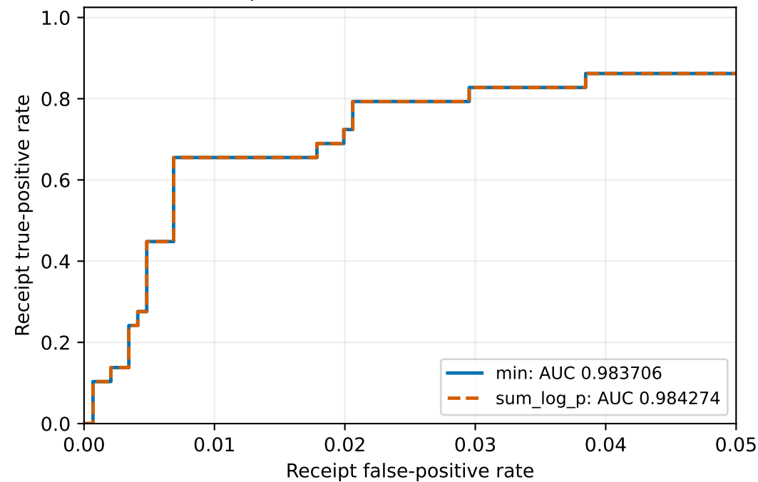
qualification — low-FPR detail
