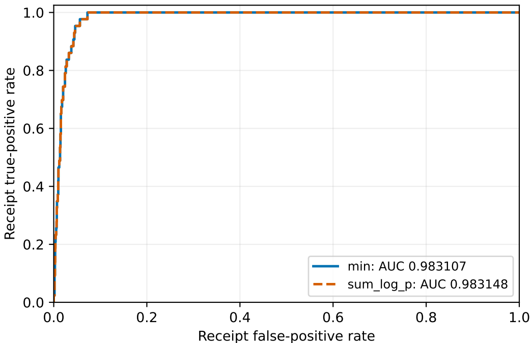
qualification — full ROC
