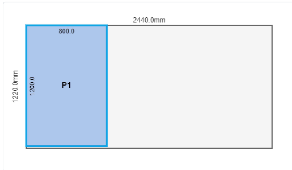
Sheet 1: Plywood1
