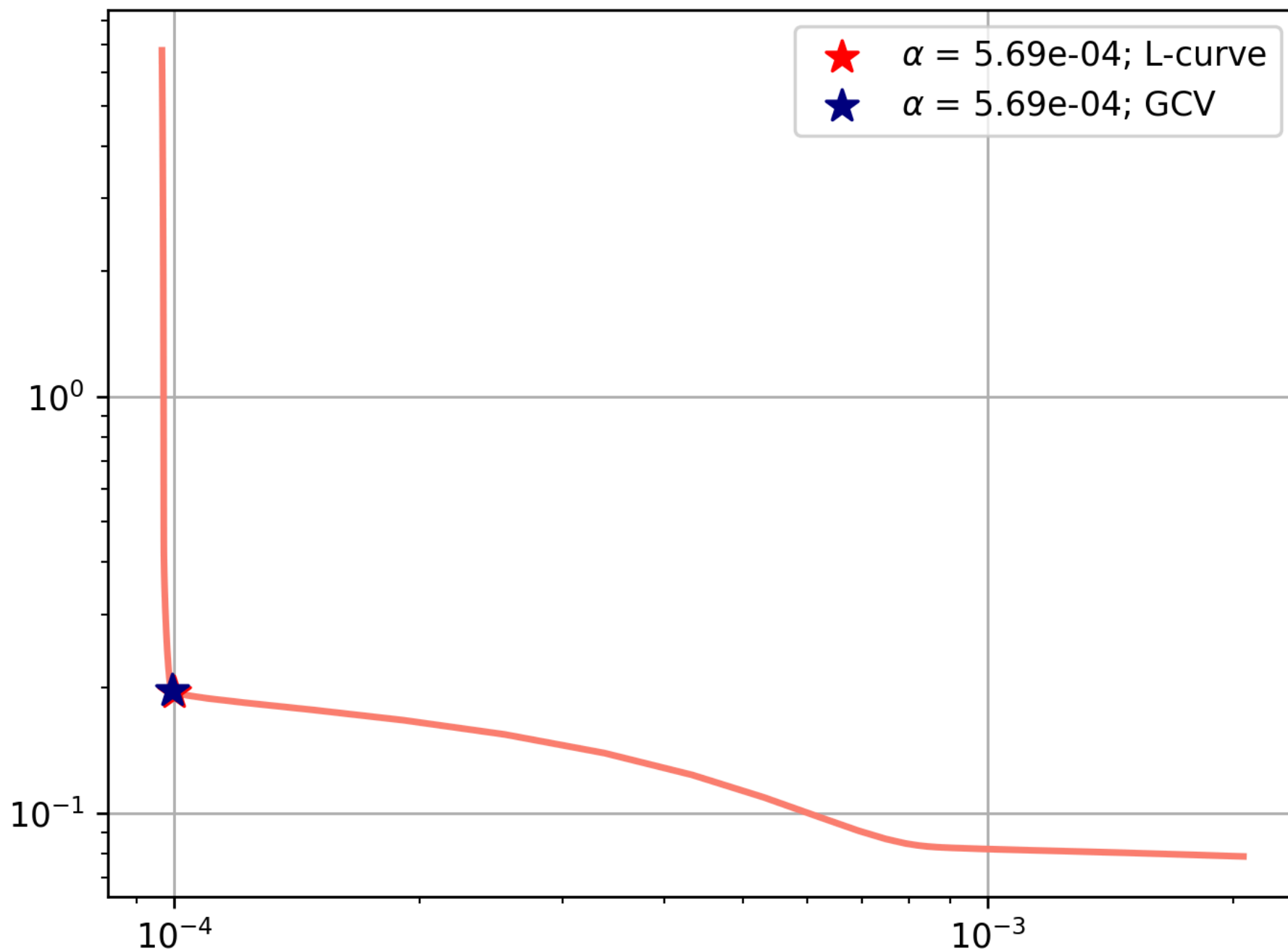
L-Curve for Second-order Tikhonov Regularization
