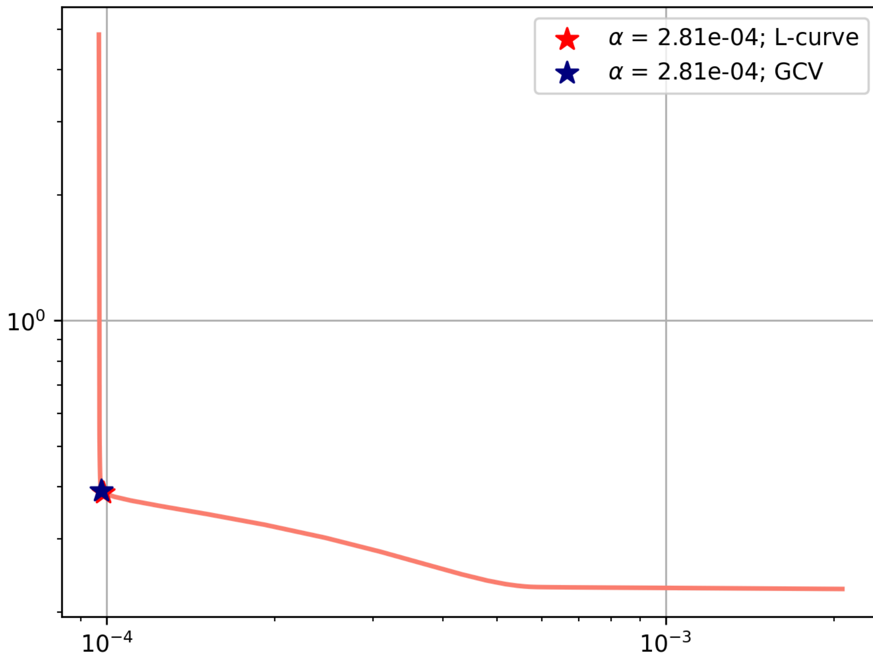
L-Curve for First-order Tikhonov Regularization
