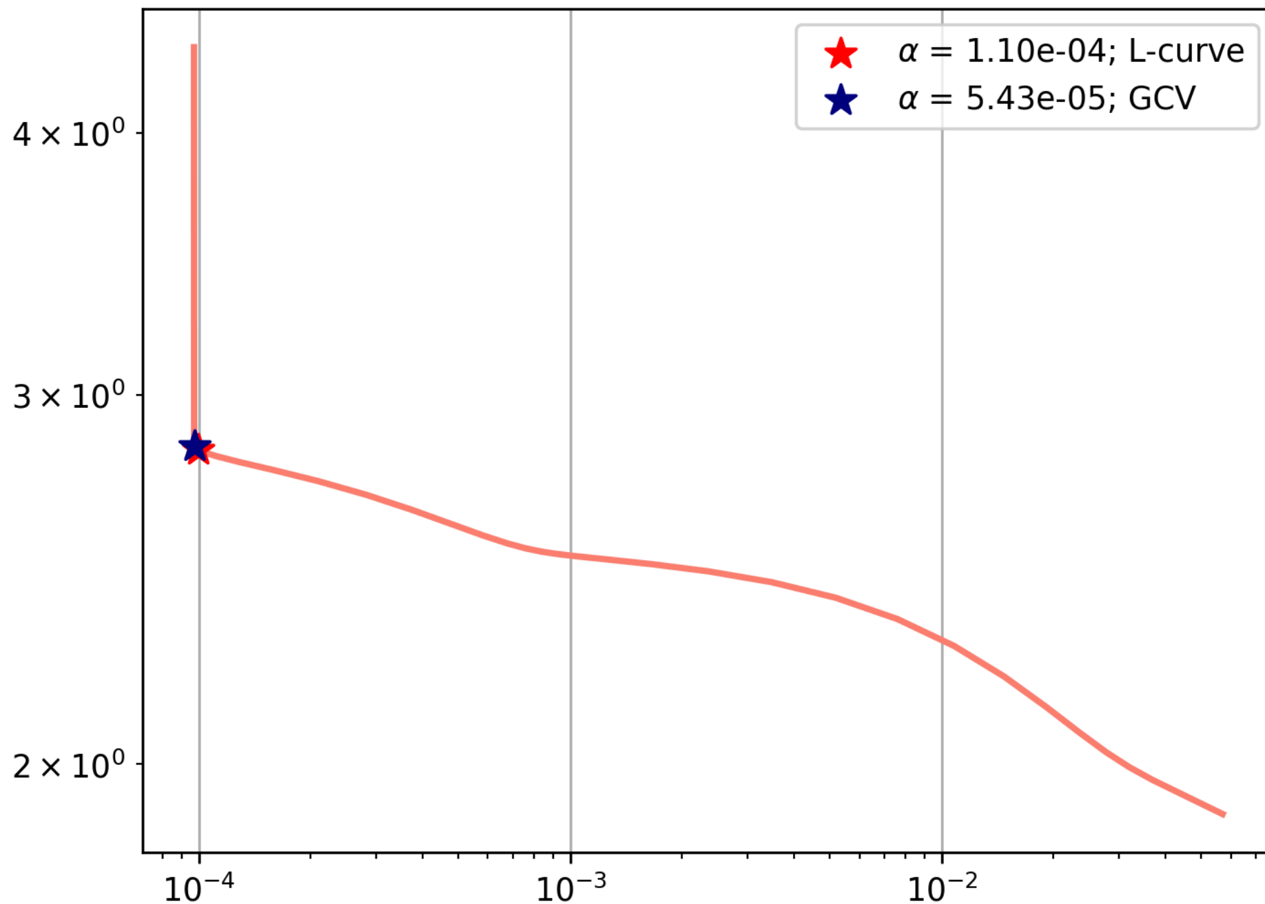
L-Curve for Zeroth-order Tikhonov Regularization
