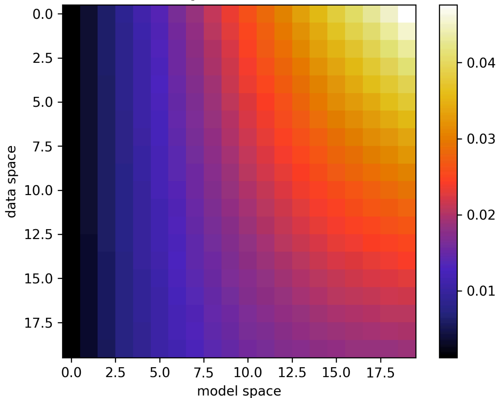
\mathcal{G} matrix from simple collocation discretization
