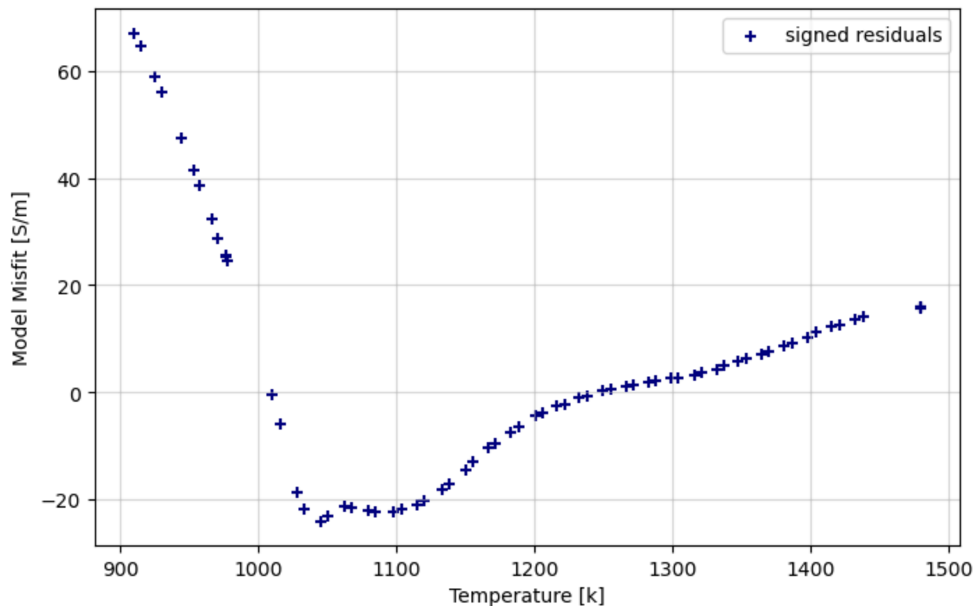
Difference between Observations and Model from Transformed LS Inversion
