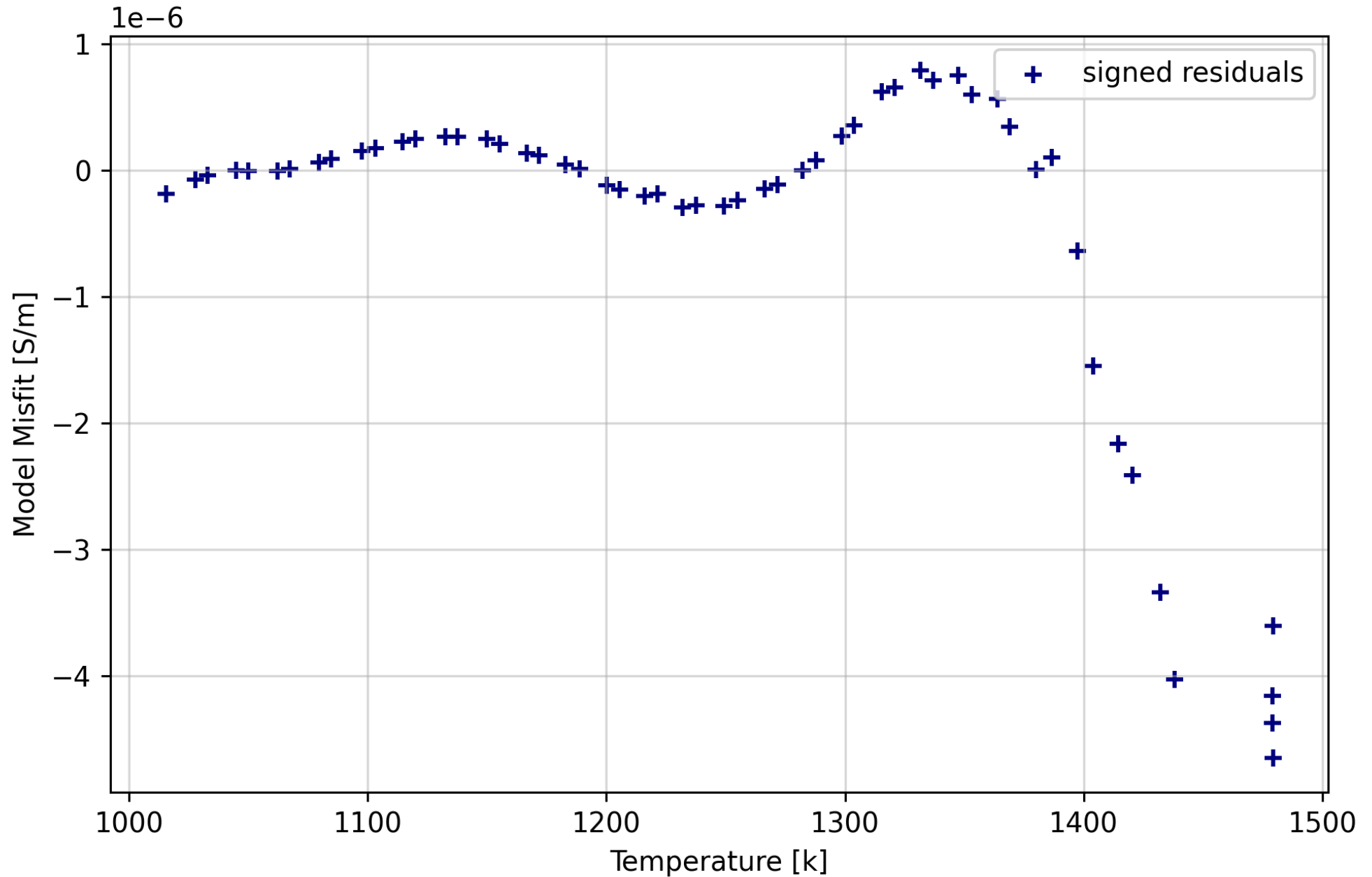
Difference between Observations and Model from Transformed LS Inversion
