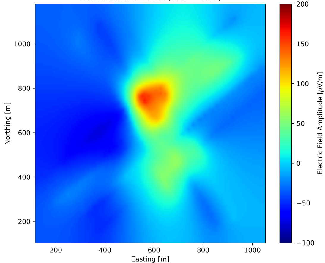
Reconstructed E-Field (RMS = 5.05)
