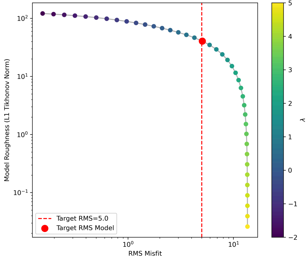
2D L-Curve Trade-off
