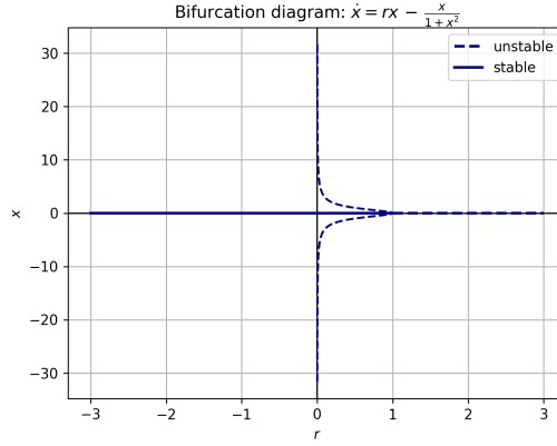
Figure 23. Bifurcation diagram for the system governed by \dot{x} = rx - \frac{x}{1+x^2} . The pitchfork bifurcation occurs moving towards r \rightarrow -\infty . The critical point is located at r_c = 1 .
