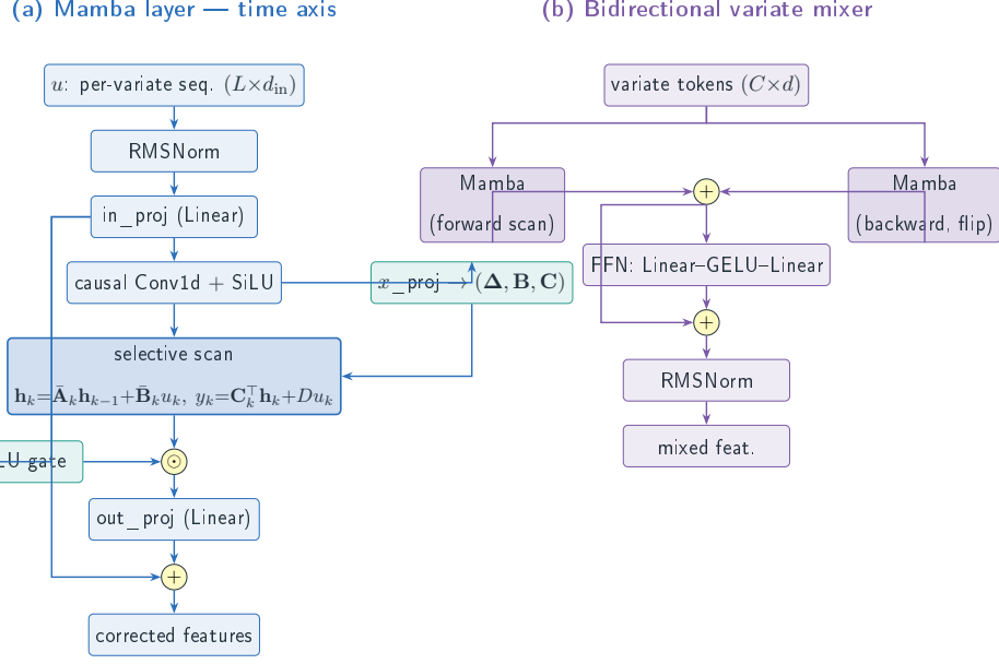
Figure 2: Internal structure of DD-Mamba’s two selective-state-space blocks (cf. the blue boxes in Fig. 1). (a) The causal Mamba layer used as the time-axis encoder (Eq. (4)): an input-dependent selective scan, gated by a SiLU branch and wrapped in a residual, with (\Delta, \mathbf{B}, \mathbf{C}) predicted per step from the input. (b) The bidirectional mixer used over the variate dimension (Section 4.3): forward and backward scans of the C channel tokens summed in one residual stream, then a position-wise feed-forward block (the S-Mamba design [7]).
