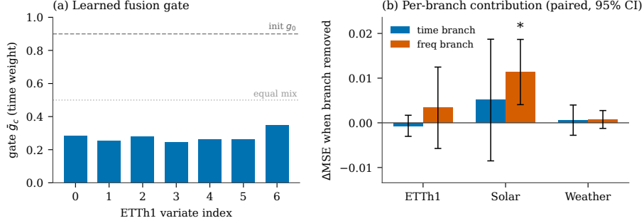
Fig. 2. Dual-domain evidence. (a) The learned fusion gate on ETTh1: the mean convex weight \bar{g}_c assigned to the time branch for each variate over the test set. Initialized time-heavy at g_0 \approx 0.9 (dashed), the trained gate redistributes weight toward the frequency branch (below the equal-mix line, dotted), matching the ETTh1 ablation in which the frequency branch alone reproduces the full model. (b) Per-branch contribution: the paired increase in MSE ( H=96 , three seeds) when each branch is removed — freq contribution = time-only – full, time contribution = freq-only – full — with t -based 95% CIs; * marks a CI clearing zero. Only Solar’s frequency branch is individually significant; on ETTh1 and Weather the branches are mutually redundant. This is the visual form of our conditional dual-domain claim: the two domains are complementary on some datasets and interchangeable on others.
