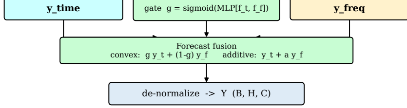
Figure 2: Forecast fusion and reconstruction. Branch features parameterize the gate g ; the two branch forecasts are then combined either convexly ( g\mathbf{Y}_t + (1-g)\mathbf{Y}_f , the default) or additively ( \mathbf{Y}_t + \alpha\mathbf{Y}_f ), and the result is de-normalized. The convex rule confines the output to the segment between the two branch forecasts; the additive rule lifts that constraint (Section 6).
