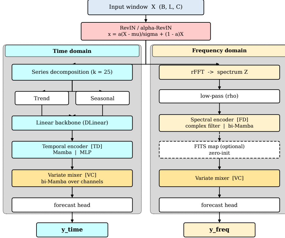
Figure 1: DD-Mamba as a forecast-decomposable architecture. The normalized input is routed to two explicit prediction paths, drawn as the shaded time-domain (left) and frequency-domain (right) bands. The time branch applies moving-average decomposition, a DLinear anchor and a temporal encoder [TD]; the frequency branch applies an rFFT, an optional low-pass, a spectral encoder [FD] and an optional FITS-style linear map (dashed: enabled per dataset). Both branches end in a cross-variate mixer [VC] and a forecast head, so each emits a complete forecast, \mathbf{Y}_t or \mathbf{Y}_f . Block labels [TD], [VC] and [FD] index the ablation grid of Table 6. Fusion and reconstruction continue in Fig. 2. Drawn to the template supplied for this submission and released as editable Visio source (fig_diagrams.vsd).
