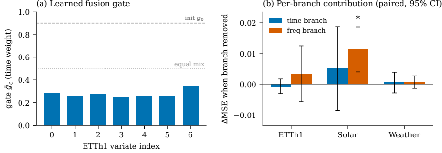
Fig. 3. Dual-domain evidence. (a) The learned fusion gate on ETTh1: the mean convex weight \bar{g}_c assigned to the time branch for each variate over the test set. Initialized time-heavy at g_0 \approx 0.9 (dashed), the trained gate redistributes weight toward the frequency branch (below the equal-mix line, dotted), matching the ETTh1 ablation in which the frequency branch alone reproduces the full model. (b) Per-branch contribution: the paired increase in MSE ( H=96 , three seeds) when each branch is removed — freq contribution = time-only – full, time contribution = freq-only – full — with t -based 95% CIs; * marks a CI clearing zero. Only Solar’s frequency branch is individually significant; on ETTh1 and Weather the branches are mutually redundant. This is the visual form of our conditional dual-domain claim: the two domains are complementary on some datasets and interchangeable on others.
