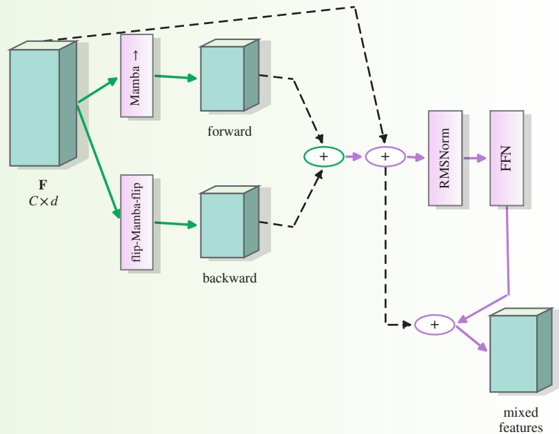
Bidirectional variate mixer
