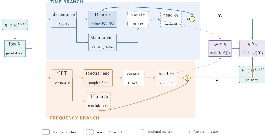
Figure 1: DD-Mamba overview. Colour encodes role — normalization (teal), time branch (blue), frequency branch (orange), and convex-gate fusion (violet) — while line style encodes trainability (legend, bottom): solid boxes are trained anchors (the DLinear backbone, spectral encoder), dashed boxes are zero-initialized corrections (the nonlinear heads \phi and the FITS map), and dotted boxes are per-dataset switches (the variate mixers). Since every correction starts at zero, the model begins as a scaled linear map of the instance-normalized window. Dotted violet arrows carry branch features to the gate, whose convex weight g mixes the two forecast paths \mathbf{Y}_{\text{time}} and \mathbf{Y}_{\text{freq}} .
