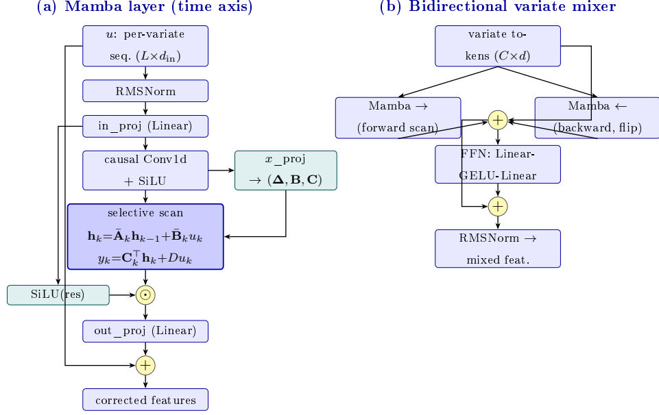
Figure 2: Internal structure of DD-Mamba’s two selective-state-space blocks (cf. the blue boxes in Fig. 1). (a) The causal Mamba layer used as the time-axis encoder (Eq. (2)): an input-dependent selective scan, gated by a SiLU branch and wrapped in a residual, with (\Delta, B, C) predicted per step from the input. (b) The bidirectional mixer used over the variate dimension (Section 3.4): forward and backward scans of the C channel tokens summed in one residual stream, then a position-wise feed-forward block (the S-Mamba design [7]).
