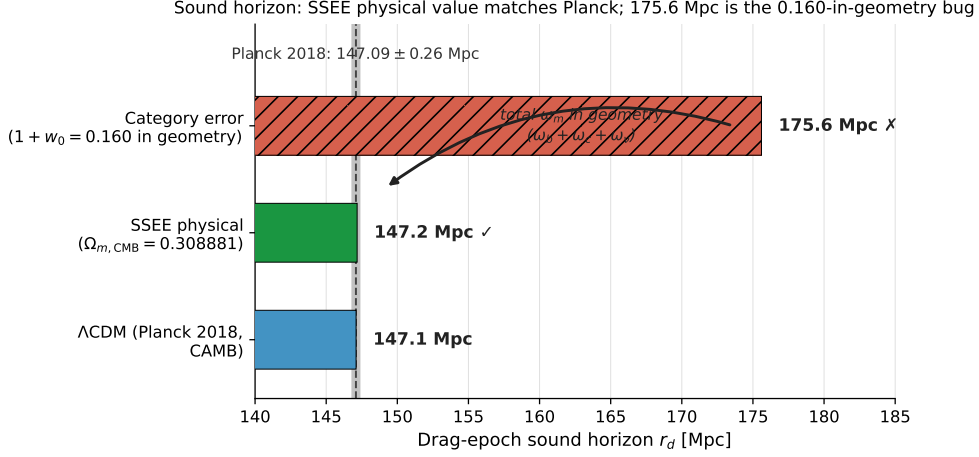
Figure 6: The physical sound horizon. Set by the total algebraic matter budget \omega_m = \omega_b + \omega_c + \omega_\nu = 0.14267 ( \Omega_m = \omega_m/h^2 = 0.308881 , \omega_m -direct, no matter factor), the SSEE drag scale is r_d = 147.17 Mpc (CAMB; log p3_rd_reframe_omega_m ), consistent with the Planck-inferred 147.09 \pm 0.26 Mpc (grey band, 0.32\sigma ) and with \Lambda CDM at the Planck 2018 parameters (147.10 Mpc, same code; log rd_dual ), a 0.05% difference. The 175.6 Mpc value that appears if the cold sector 1 + w_0 = 0.160050 is (incorrectly) used as the background density is a category error, not a physical scale.
