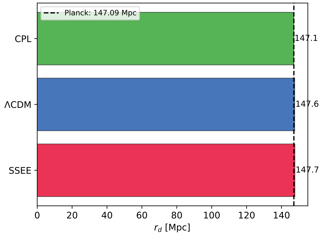
Sound horizon r_d (MAP) — SSEE matches \Lambda CDM
