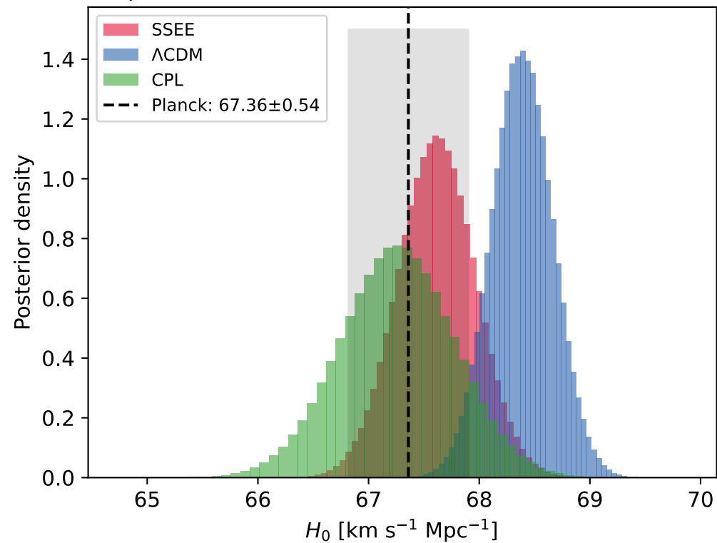
H_0 posteriors — SSEE 67.62 \pm 0.35 ( 0.40\sigma Planck)
