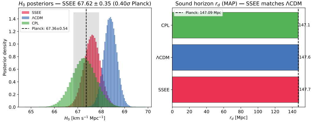
Figure 5: Left : H_0 posteriors for all three models under a common Planck prior (the apples-to-apples model-comparison run); the SSEE posterior sits at 67.62 \pm 0.35 , 0.40\sigma from Planck 2018 and fully consistent with the titular algebraic-anchor-prior value 67.82 \pm 0.41 ( 0.68\sigma Planck, 0.34\sigma from H_0^{\text{glob}} = 67.962 ). Right : MAP r_d values; the SSEE sound horizon ( 147.7 \text{ Mpc} ) matches \Lambda\text{CDM} ( 147.6 \text{ Mpc} , ratio 1.0008), CAMB with each model’s own m_\nu .
