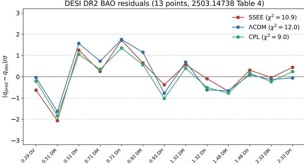
Figure 8: Normalised BAO residuals (q^{\text{pred}} - q^{\text{obs}})/\sigma for all 13 DESI DR2 measurements. SSEE (red), \Lambda CDM (blue), CPL (green). With the total matter density the SSEE sound horizon ( r_d = 147.17 Mpc, CAMB) matches \Lambda CDM, and the residuals are comparable across models, quantified in the \chi^2_r values of Section 8.
