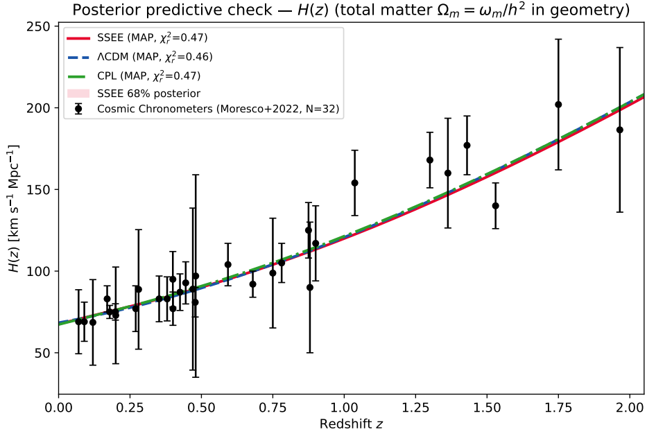
Figure 7: MAP H(z) vs the 32 Cosmic Chronometers of Table 7 [Jimenez & Loeb, 2002, Moresco et al., 2022]. Red band: SSEE 68% posterior interval.
