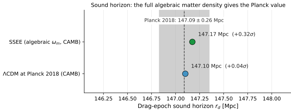
Figure 6: The physical sound horizon. Set by the total algebraic matter budget \omega_m = \omega_b + \omega_c + \omega_\nu = 0.14267 ( \Omega_m = \omega_m/h^2 = 0.308881 , \omega_m -direct, no matter factor), the SSEE drag scale is r_d = 147.17 \text{ Mpc} (CAMB, green), consistent with the Planck-inferred 147.09 \pm 0.26 \text{ Mpc} (grey band, 0.32\sigma ) and with \Lambda\text{CDM} at the Planck 2018 parameters ( 147.10 \text{ Mpc} , same code, blue). Log rd_dual .
