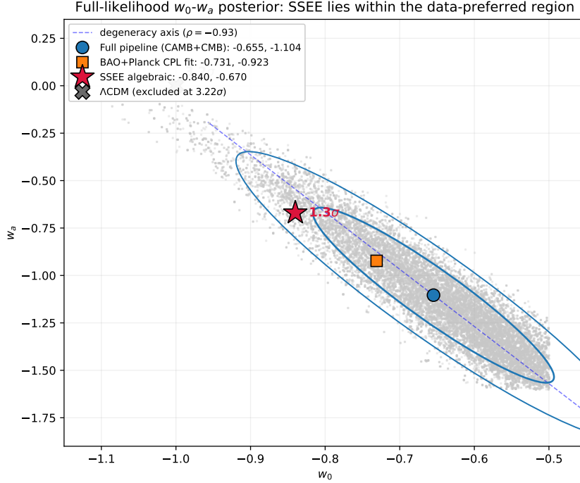
Figure 9: Full-likelihood w_0 - w_a posterior (CAMB + Planck plik_lite + lensing + DESI DR2 + f\sigma_8 , with w_0, w_a free; R - 1 < 0.003 ). The SSEE algebraic prediction (red star) lies at 1.31\sigma , inside the 2\sigma contour, while \Lambda CDM ( w_0 = -1, w_a = 0 ; grey cross) is excluded at 3.22\sigma . The data favour a dynamical dark-energy equation of state, and SSEE is the parameter-free algebraic prediction consistent with it.
