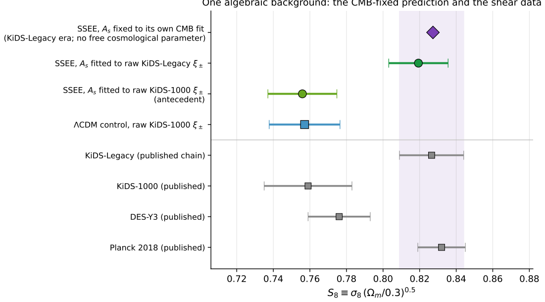
Figure 3: S_8 on the algebraic background of SSEE, identical in every SSEE row; only the dataset asked to fix A_s changes. Purple diamond: the prediction with A_s fixed to the model’s own CMB fit — no free cosmological parameter — S_8 = 0.8273 , 0.04\sigma from the KiDS-Legacy posterior ( 0.8265 \pm 0.0176 , purple band). Green: A_s fitted to the raw KiDS-Legacy \xi_{\pm} ( 0.8193 \pm 0.0162 ) and, as antecedent, to the raw KiDS-1000 \xi_{\pm} ( 0.7559 \pm 0.0189 , 0.10\sigma from KiDS-1000). Blue: the \Lambda CDM control on the same raw KiDS-1000 data ( 0.7571 \pm 0.0194 ). Grey: published KiDS-Legacy, KiDS-1000, DES-Y3 and Planck 2018 constraints with 1\sigma errors. The shift between the two KiDS releases is in the data, not in the model.
