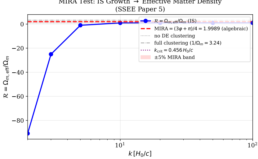
Figure 2: \mathcal{R}(k) \equiv \Omega_{m,\text{eff}}/\Omega_m (blue points with error bars) versus k/(H_0/c) ; earlier versions of this text, and of the figure axis, wrote this quantity \text{MIRA}_{\text{num}} and divided by s_m = 1+w_0 (then written \Omega_{m,\text{dyn}} ) in the label while the code already divided by \Omega_m . The former target \text{MIRA} = (3\varphi + \pi)/4 \simeq 1.999 (red dashed) is not approached: IS suppression drives \mathcal{R} \rightarrow 1 for k \gg H_0/c . The grey dash-dotted line marks full DE clustering ( \mathcal{R} = 1/\Omega_m ; an earlier caption gave 1/s_m \simeq 6.25 , which is not a clustering limit), ruled out by all current observations. The required perturbation amplitude r^* = 0.190 (Eq. 30) would require DE clustering at the 19% level — not produced by IS dynamics. The conclusion stands: MIRA is not reproduced by IS dynamics, at either level — linear perturbations give \mathcal{R} \approx 1 and the background IS Friedmann integration a ratio \approx 3.04 , neither of them 1.9989. Both figures are recorded here as the historical closing of a route that is no longer open: the target 1.9989 was the matter factor \Omega_{m,\text{CMB}} = \text{MIRA} \times \Omega_{m,\text{dyn}} , withdrawn on 2026-06-18 when OP-8 closed. MIRA survives as the screening entity of Paper 9, where it is not a matter factor and nothing here bears on it. See Section 7.1.
