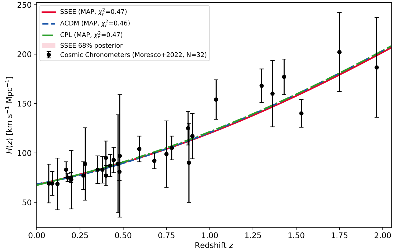
Posterior predictive check — H(z) (total matter \Omega_m = \omega_m/h^2 in geometry)
