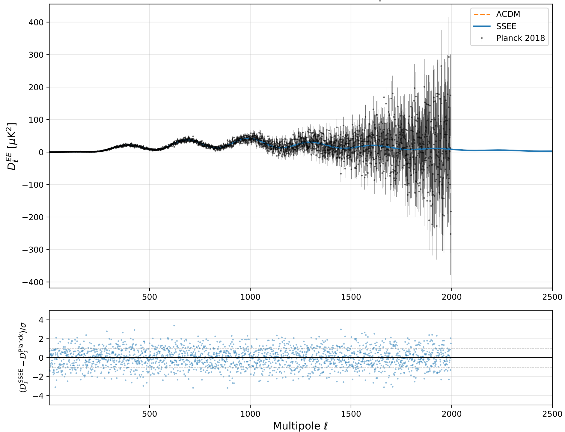
SSEE vs Planck 2018: CMB EE Power Spectrum
