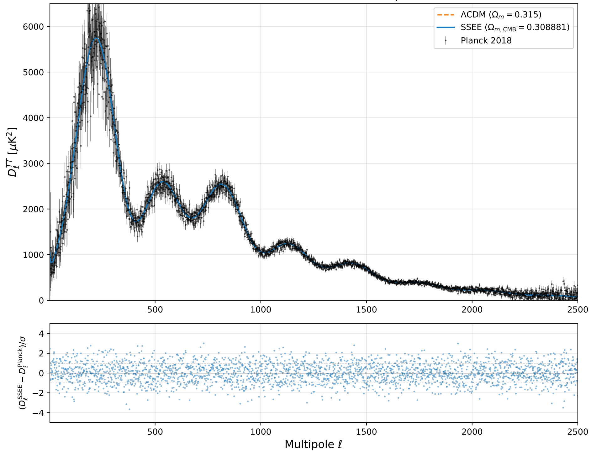
SSEE vs Planck 2018: CMB TT Power Spectrum
