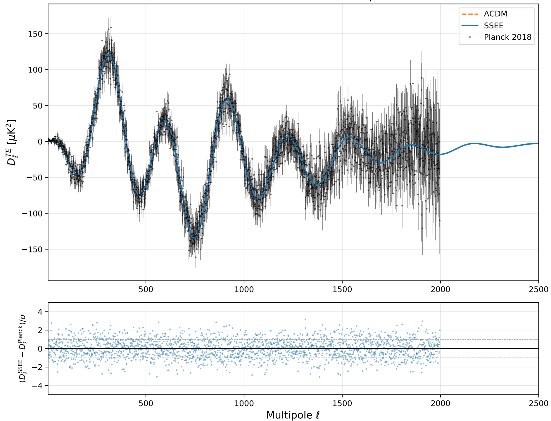
SSEE vs Planck 2018: CMB TE Power Spectrum
