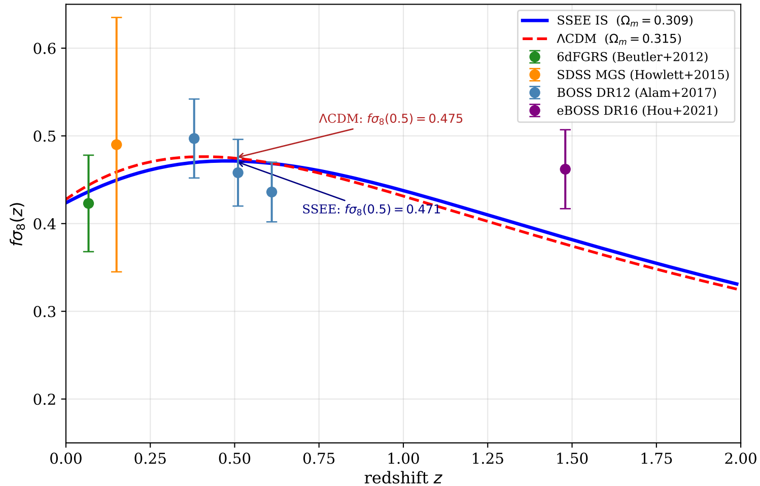
f\sigma_8(z) : SSEE IS vs \Lambda CDM vs RSD data
