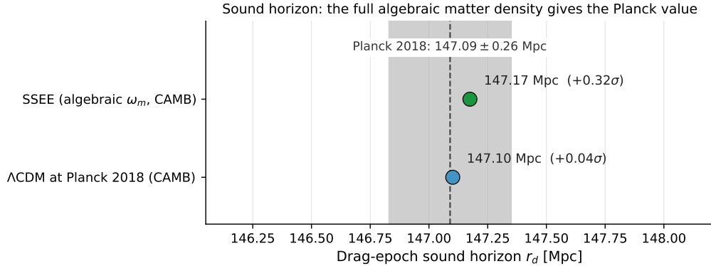
FIG. 2. The physical sound horizon. Set by the full algebraic \omega_m (green, 147.17 Mpc at \Omega_m^{\text{cosm}} = 0.308881 , \omega_m -direct), in agreement with Planck 2018 ( 147.09 \pm 0.26 Mpc, grey band) and with \Lambda\text{CDM} at the Planck 2018 parameters (blue, 147.10 Mpc, CAMB). This is the visual counterpart of the Boltzmann test above: the full matter density that restores the acoustic peaks also restores the BAO standard ruler.
