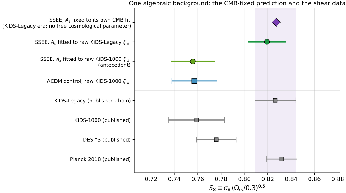
FIG. 5. S_8 on the algebraic background of SSEE, identical in every SSEE row; only the dataset asked to fix A_s changes. Purple diamond: the prediction with A_s fixed to the model’s own CMB fit — no free cosmological parameter — S_8 = 0.8273 , 0.04\sigma from the KiDS-Legacy posterior ( 0.8265 \pm 0.0176 , purple band). Green: A_s fitted to the raw KiDS-Legacy \xi_{\pm} ( 0.8193 \pm 0.0162 ) and, as antecedent, to the raw KiDS-1000 \xi_{\pm} ( 0.7559 \pm 0.0189 , 0.10\sigma from KiDS-1000). Blue: the \Lambda CDM control on the same raw KiDS-1000 data ( 0.7571 \pm 0.0194 ). Grey: published KiDS-Legacy, KiDS-1000, DES-Y3 and Planck 2018 constraints with 1\sigma errors. The shift between the two KiDS releases is in the data, not in the model.
